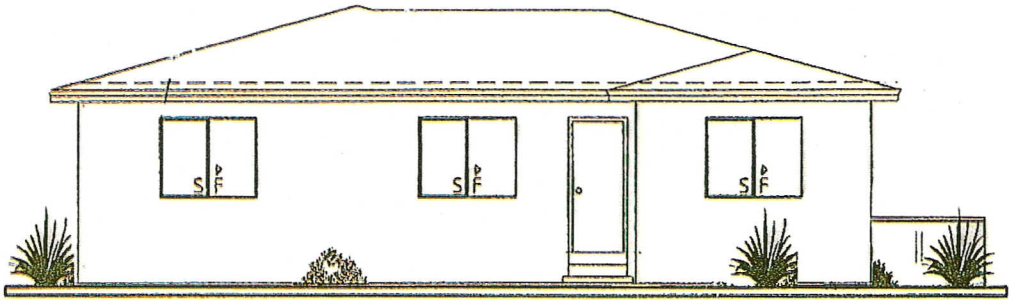
FRONT ELEVATION
