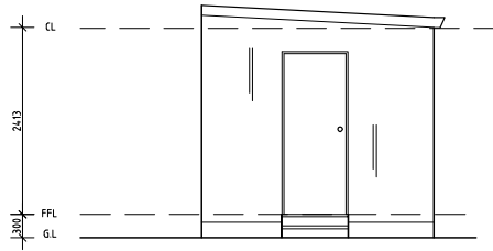
END ELEVATION 1 SCALE 1:100
